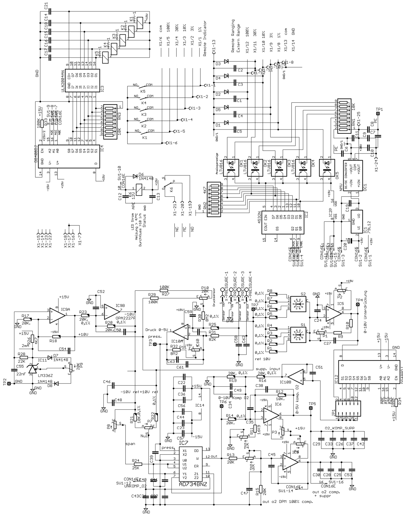
Figure 15 Circuit diagram extension board PMA 30
