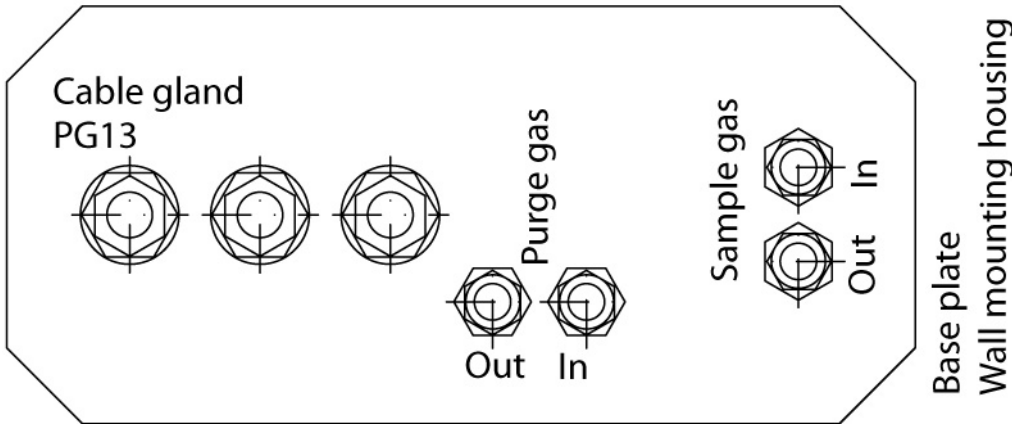
Figure 17 Connections wall mounting housing PMA 30
