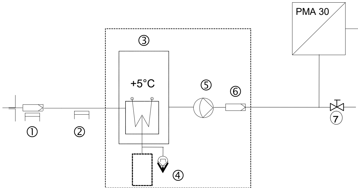
Figure 5 Standard gas conditioning system
