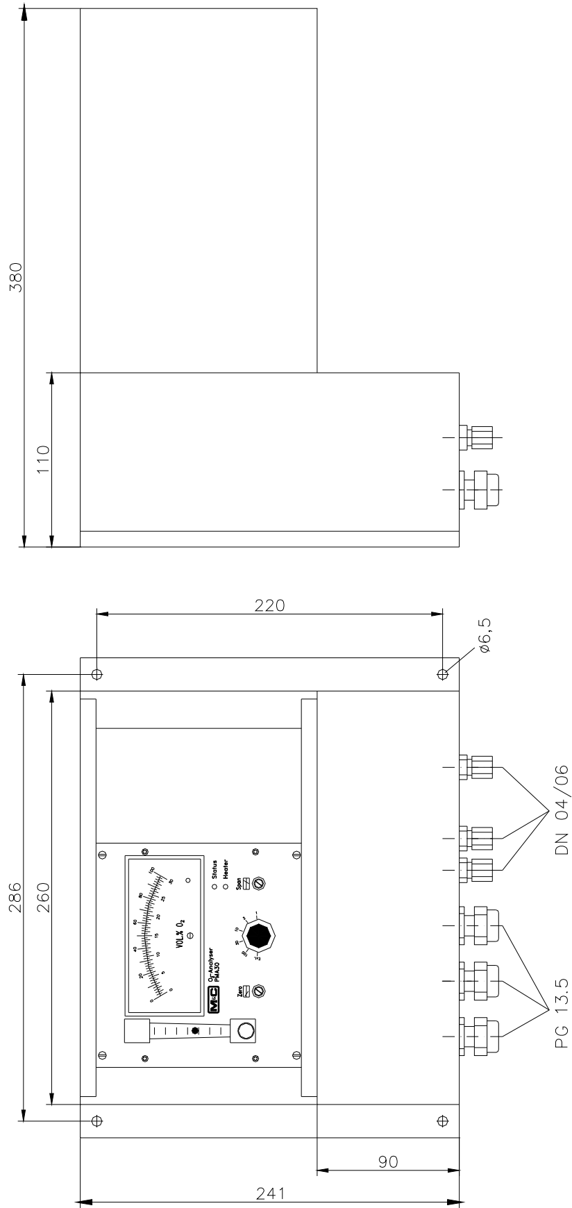
PMA 30 in wall mounting housing
