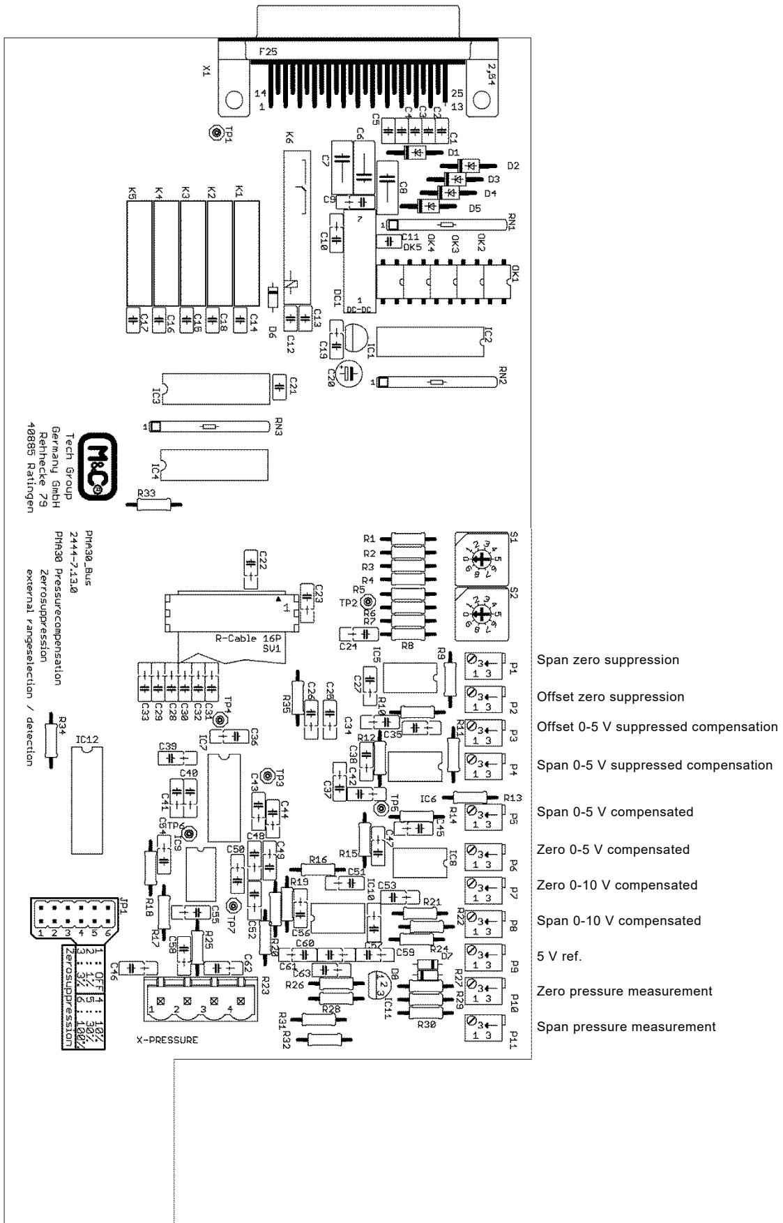
Figure 16 Assembly diagram extension board PMA 30
