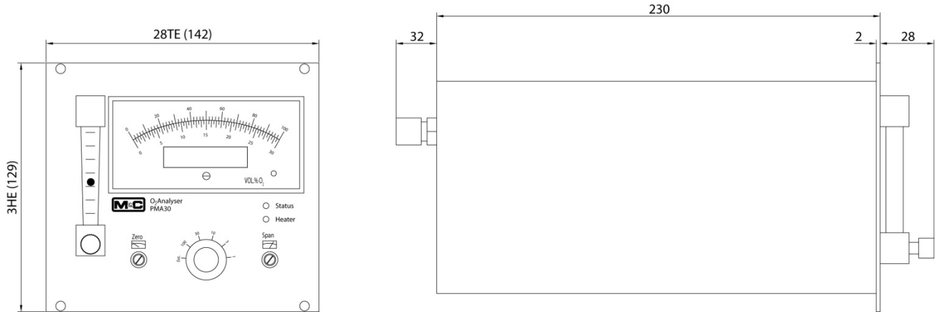
Figure 1 Dimensions PMA30
