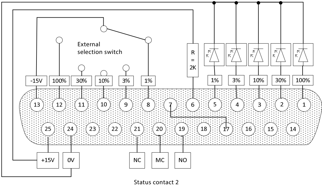
Figure 8 Pin assignment of D-sub-connector X1
