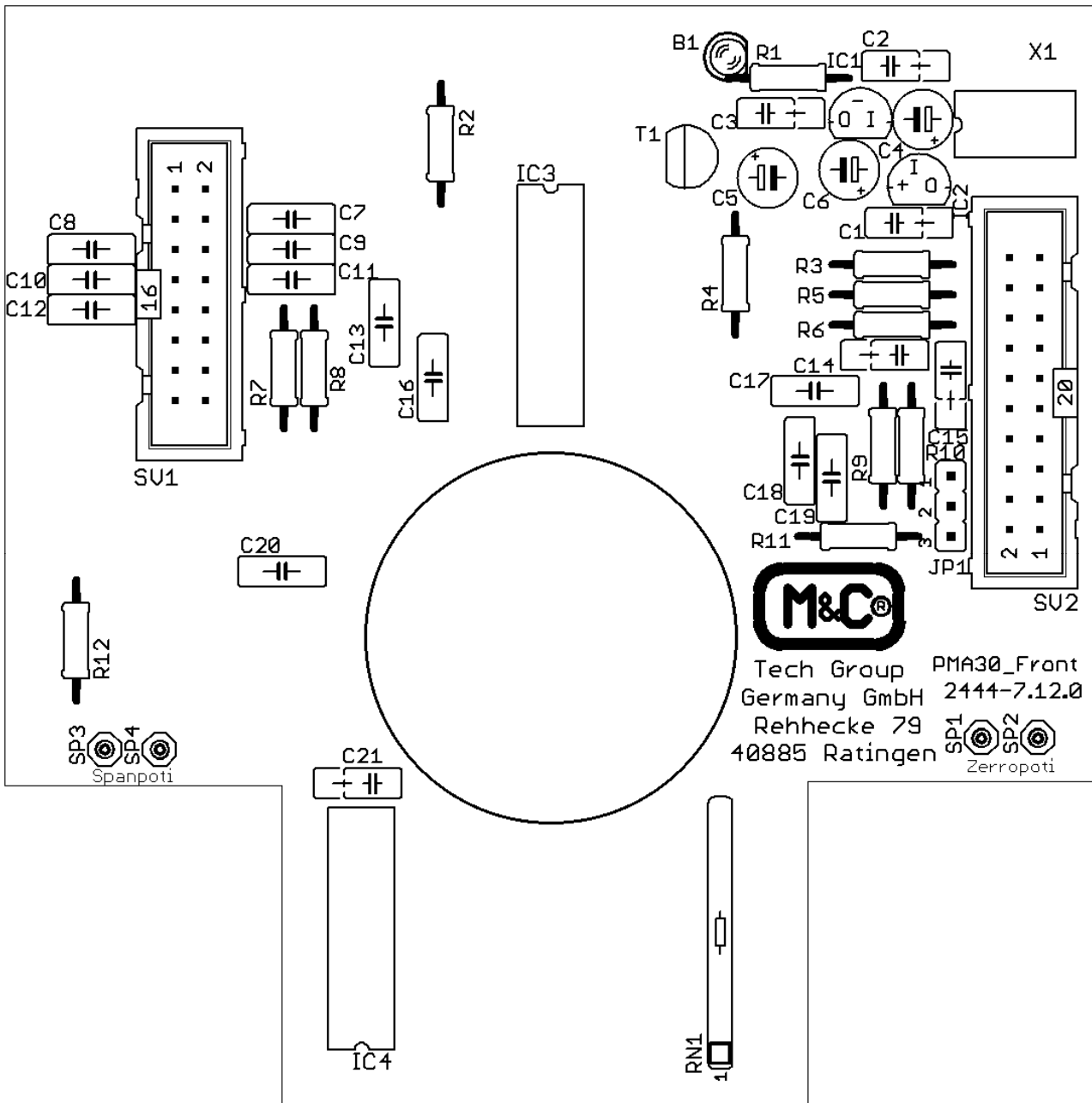
Figure 14 Assembly diagram front board PMA 30
