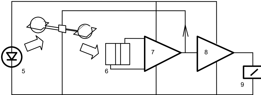
Figure 3 Scheme of the measuring cell and optical signal processing
