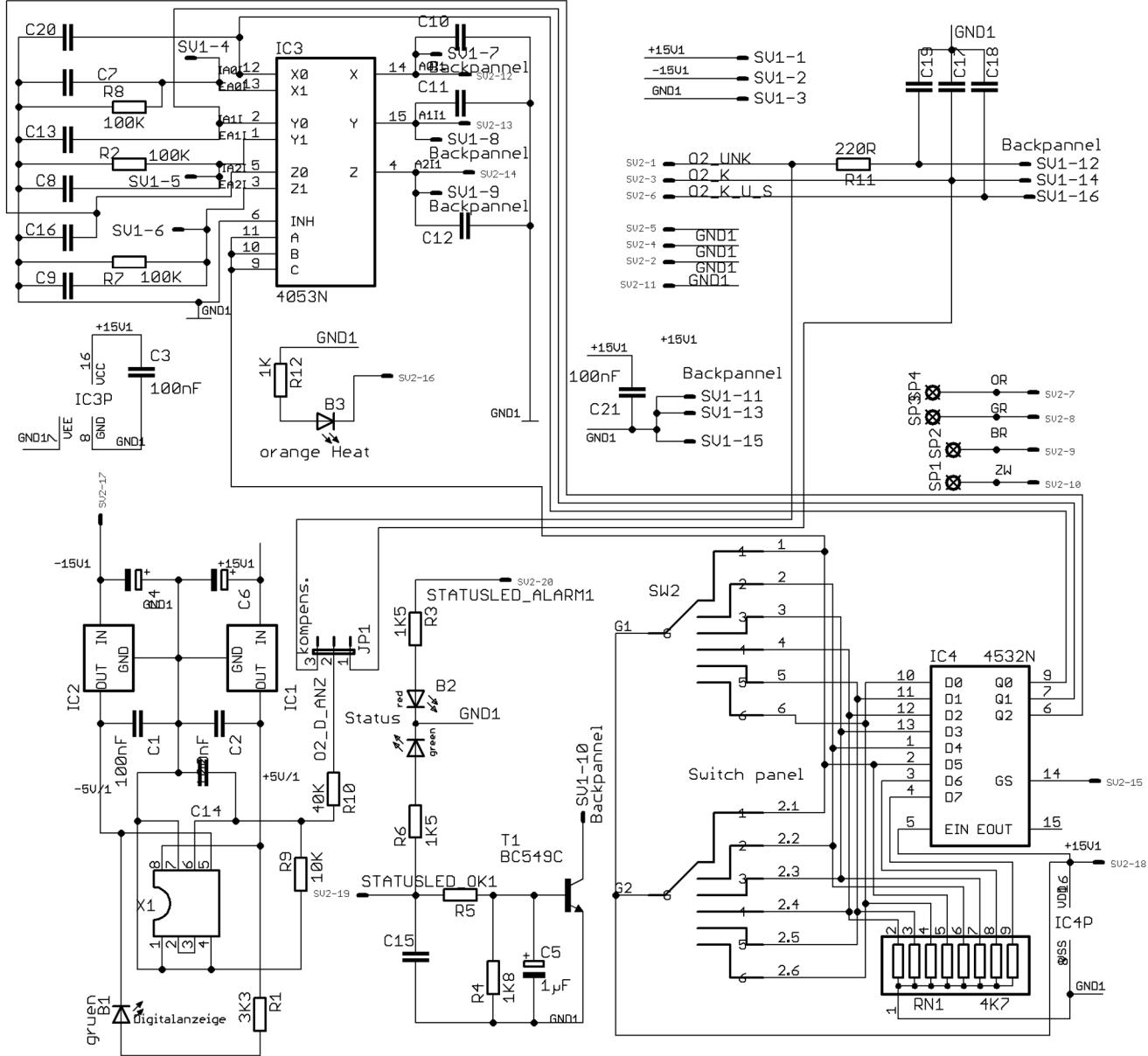
Figure 13 Circuit diagram PMA 30 front board
