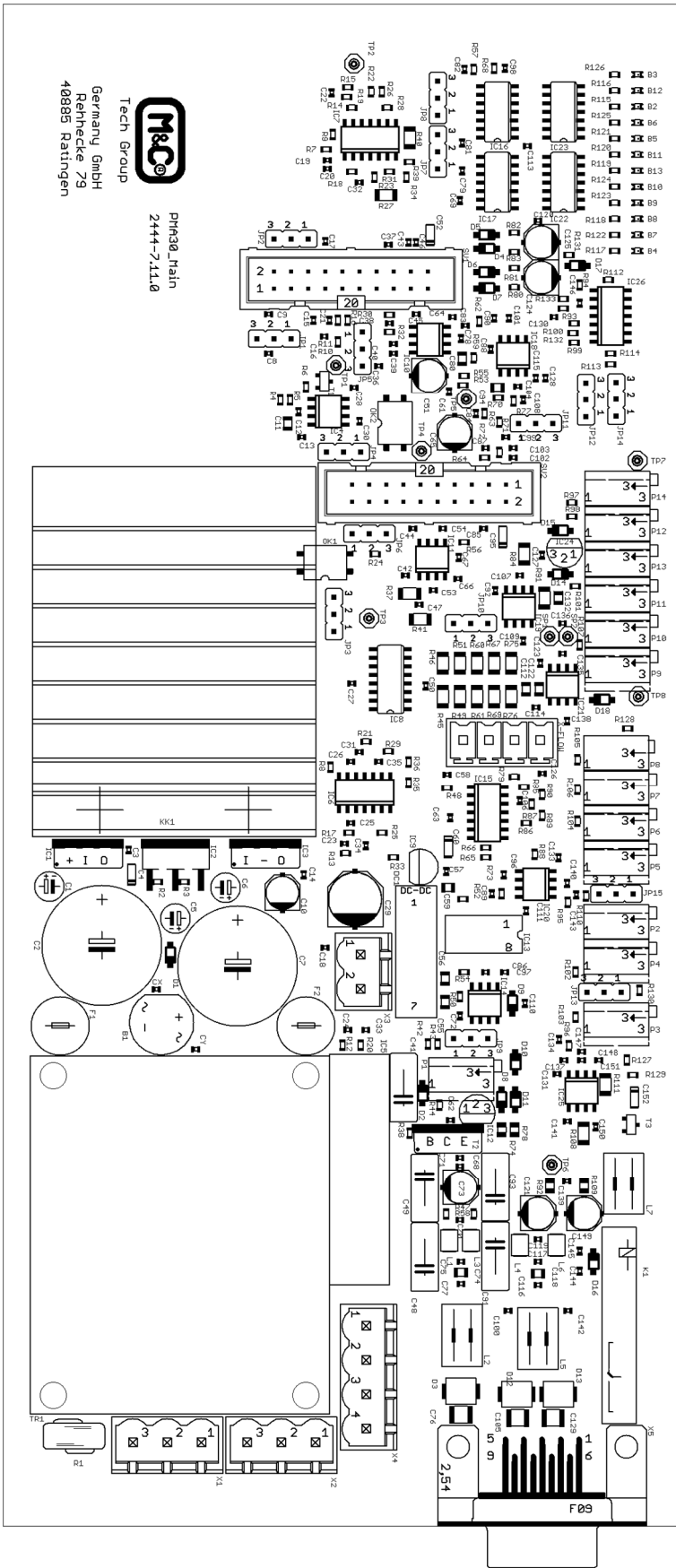
Figure 12 Assembly diagram PMA 30 main board
