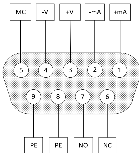
Figure 7 Pin assignment of D-sub-connector X4
